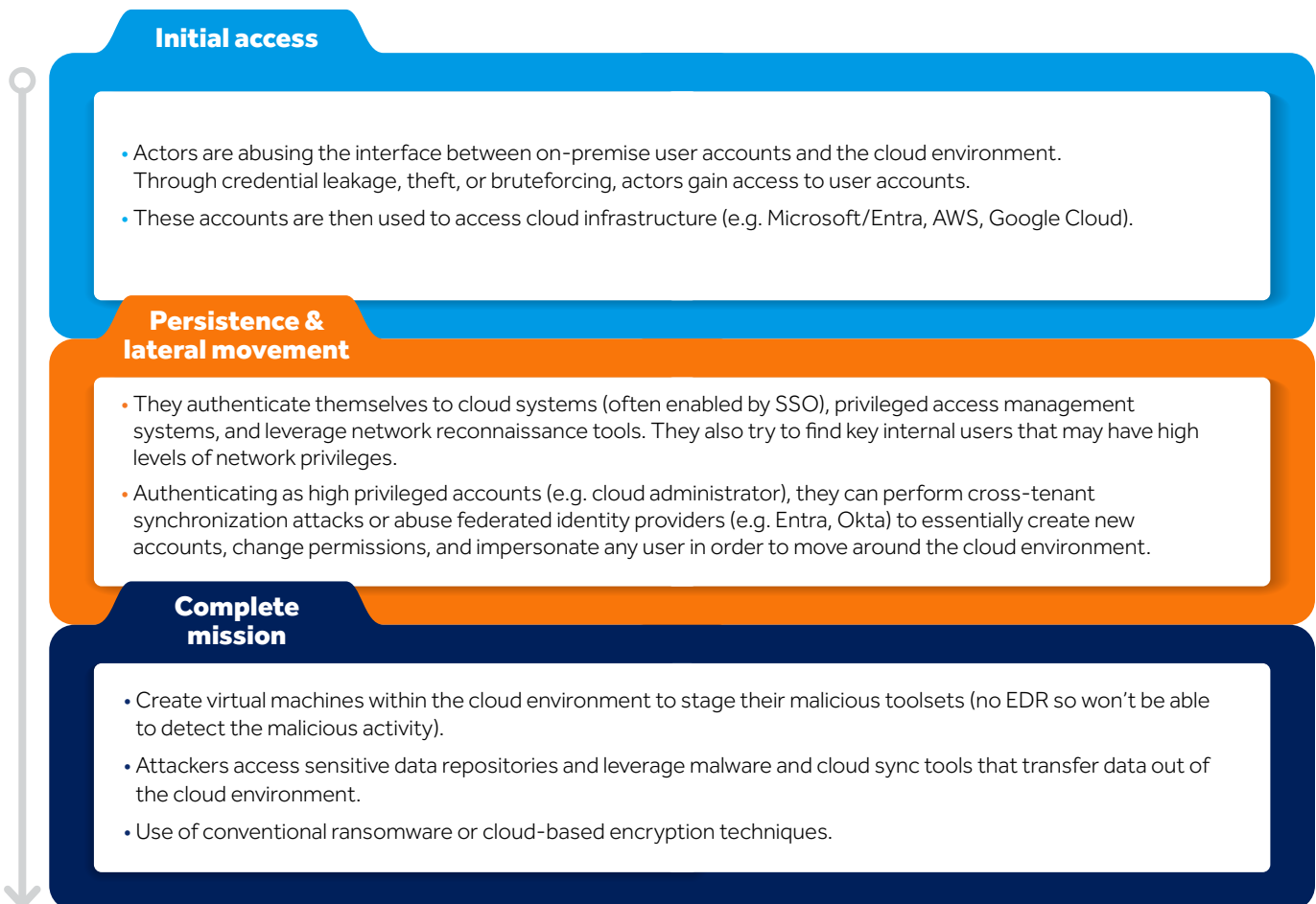
Figure 1: High-level attack flow of how cloud attacks are materialising
